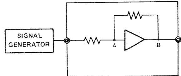
Figure 6— Negative Feedback Amplifier Gain Measurement.
